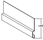
FASCIA APRON, RECTANGULAR RT412 COLORS: WHITE, ALMOND, DESERT SAND, EVERGREEN, MUSKET BROWN, PEBBLESTONE CLAY, SANDTONE, TERRA BRONZE, VICTORIAN GREY
